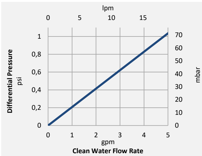
Graph 1: Z.Plex Filterplex.Z Depth Filter clean water flow rate based on a 10 in length filter. One line for both micron ratings.
